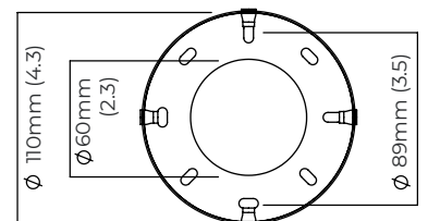
mounting plate dimensions
